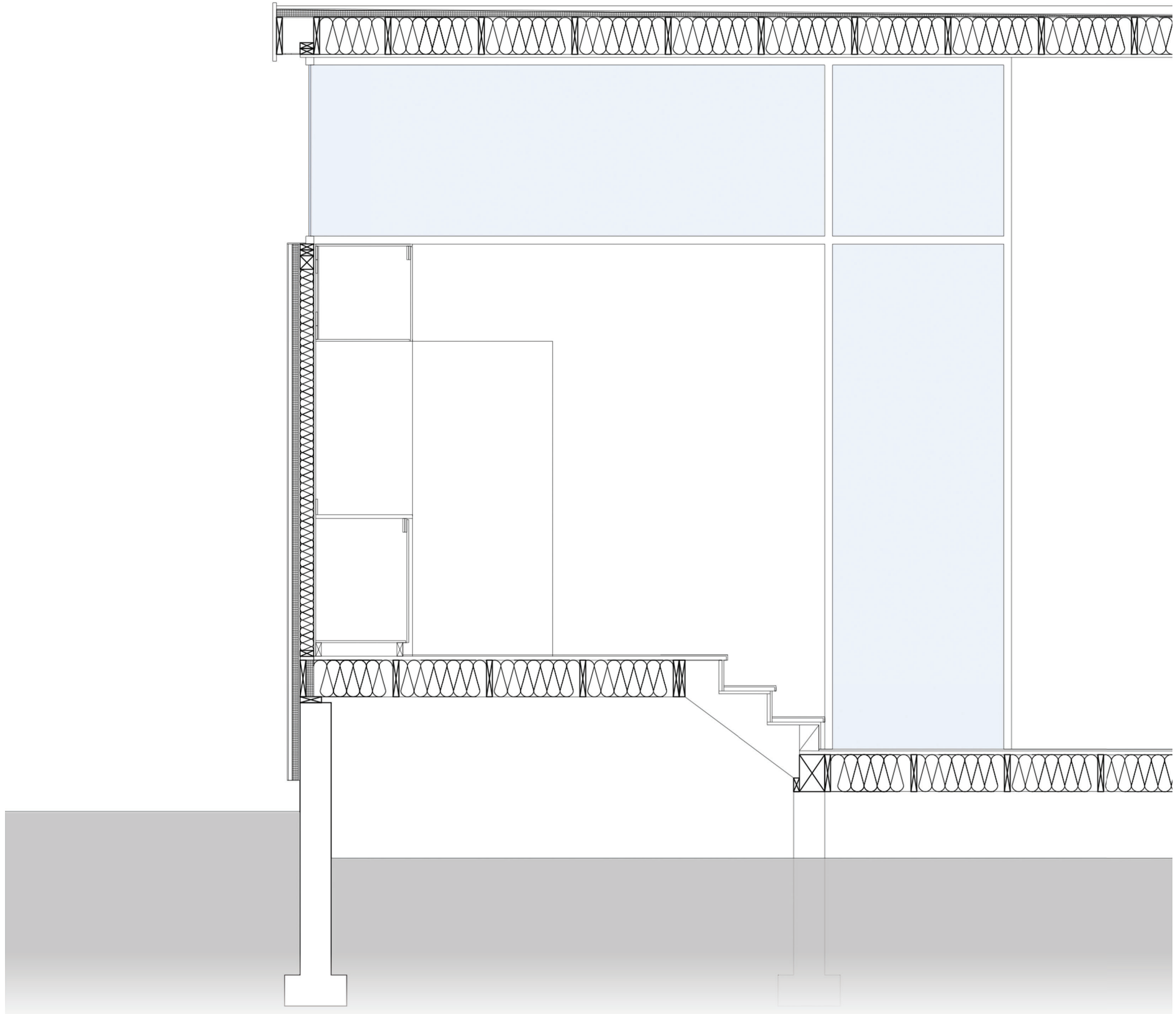
Detailed Section 1/2" = 1' 0"
